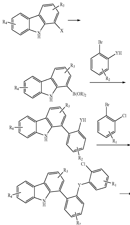
[Reaction Scheme 1]
